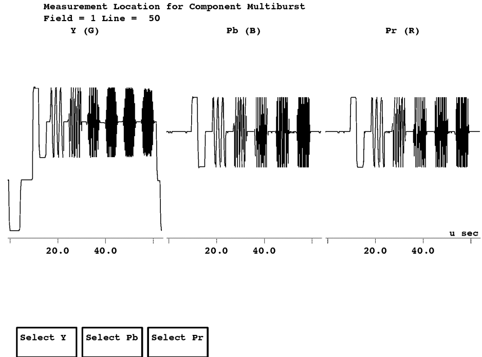
Figure 2-20: MultiBurst special position display
